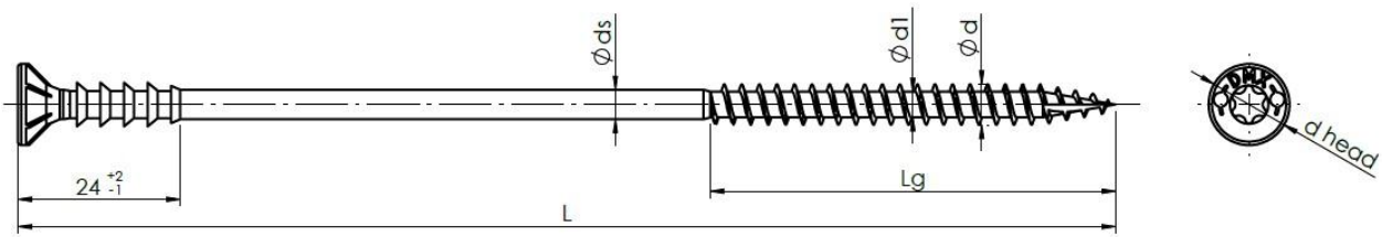
Figure 3 Screw, type WDS
