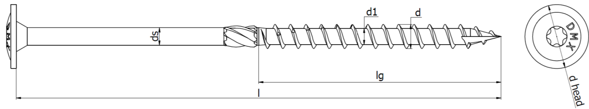
Figure 2 Screw, type CT
